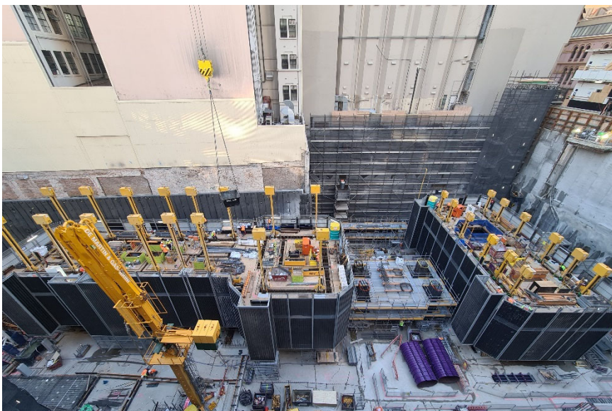
Pitt Street North site: view of the east and west jumpform use to build the core building structure
